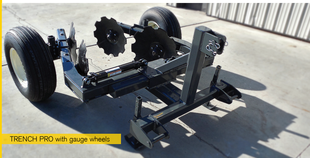
Hydraulically adjustable width
